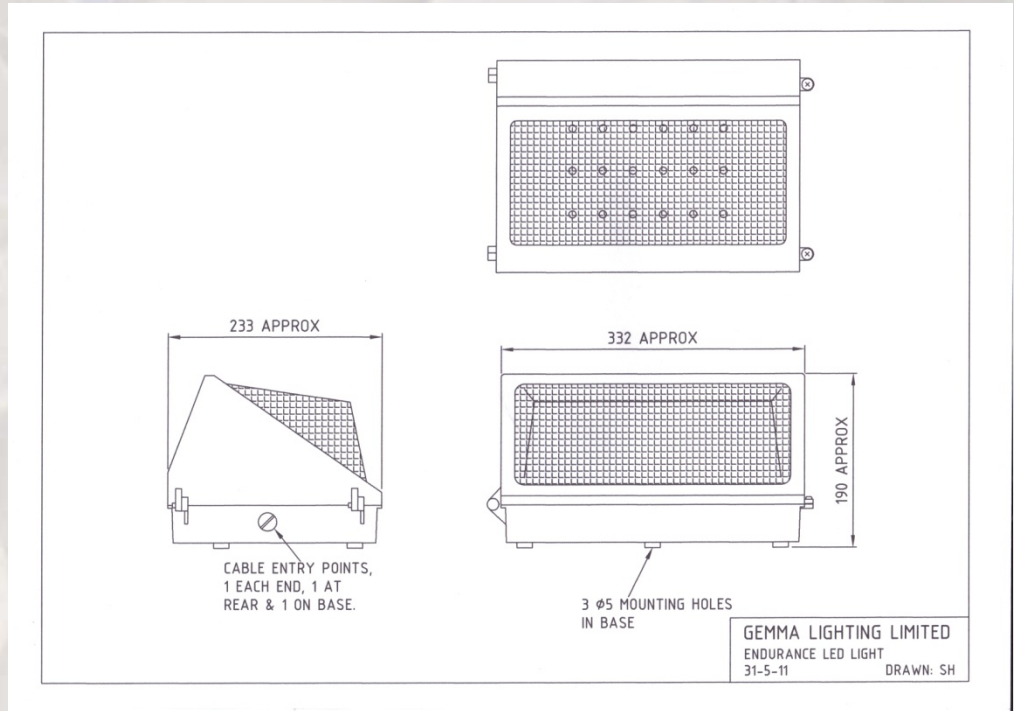
Above: CAD diagram for Endurance 24 XL110 – LED Path Light
