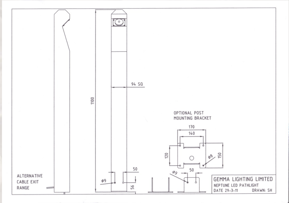
Above: CAD diagram – Neptune 5 LED Path Marker
