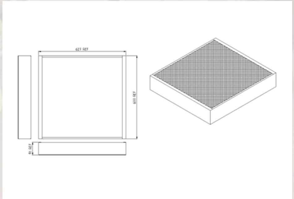
Above: CAD diagram for Venus 24 XL110 (600 X 600) LED Ceiling Tile – Surface Mount
