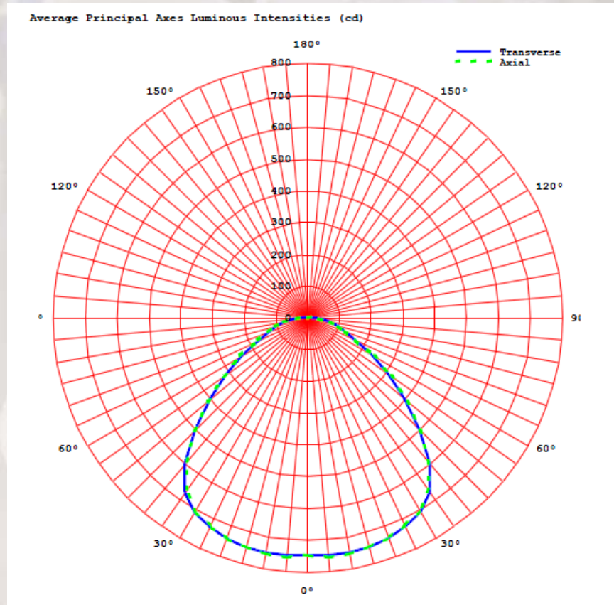
Abve: Polar plot of the Venus 24 XL110 (600 X 600) LED Ceiling Tile. Measured in candela per kilolumens.
