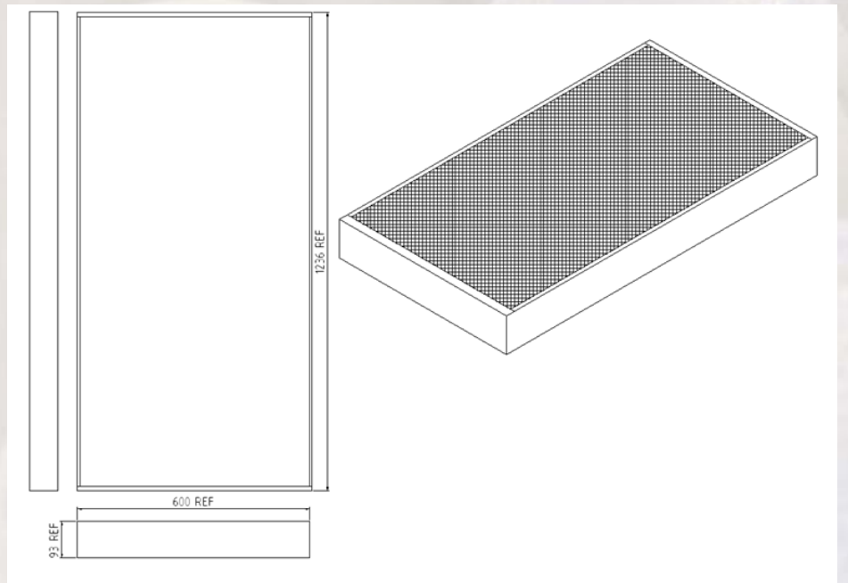
Above: CAD diagram for Venus 48 XL110 (1200 X 600) LED Ceiling Tile – Surface Mount
