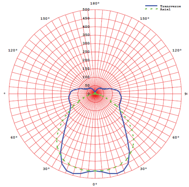
Average Principal Axes Luminous Intensities (cd)
