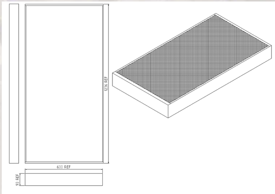
Above: CAD diagram for Venus 64 XL110 (1200 X 600) LED Ceiling Tile – Surface Mount
