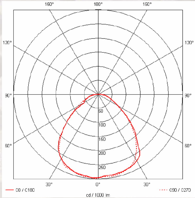
Above: Polar plot of the Venus 32 XL110 (600 X 600) LED Ceiling Tile. Measured in candela per kilolumens.
