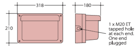
Fixing points: 4 x 7mm dia. concealed holes on 290 x 150mm centres
