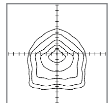
Optic 2 - IESNA Type V (circular 360°) beam for wide area lighting such as car parks.
